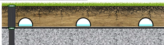
AMP-Arched Mesh Pipe System-Green Roof
