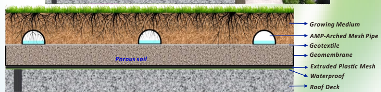
Self Watering Wicking Beds-Green Roof
